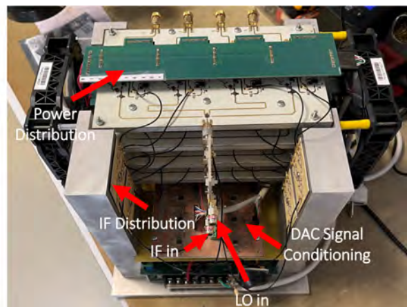
FIGURE 18. Photograph of the transmitter and its sub-components front and back of the transmitter setup as presented in [37].
