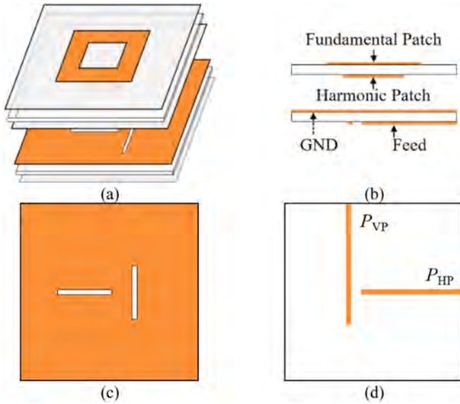
FIGURE 29. Layout of the DLP antenna presented in [160]: (a) exploded view, (b) stack-up, (c) ground layer and (d) feeding layer © IEEE 2021.
