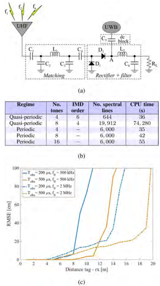
FIGURE 26. (a) Schematic representation of the passive, UWB-pulse generator tag proposed in [157], (b) comparison of computational time for periodic and quasi-periodic analysis and (c) localization RMSE for increasing TX-RX distance [157] © IEEE 2018.
