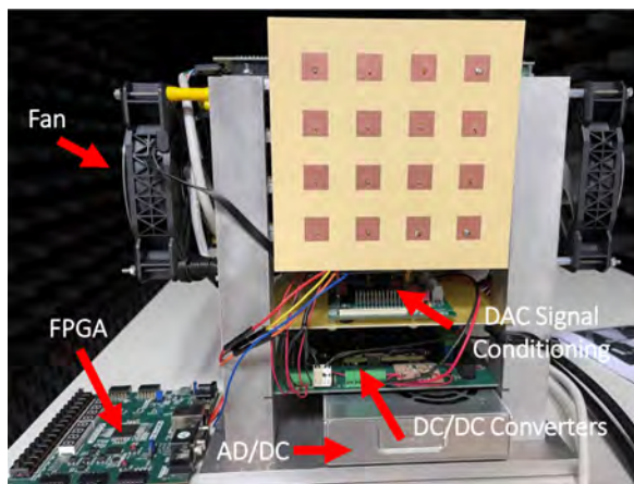
FIGURE 18. Photograph of the transmitter and its sub-components front and back of the transmitter setup as presented in [37].
