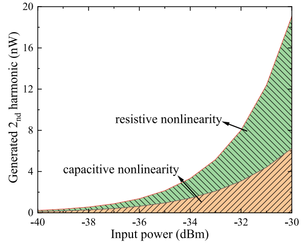
FIGURE 11. Contribution comparison of nonlinear junction resistance and capacitance during second-harmonic generation for a Schottky diode SMS7630 at 3.5 GHz. Note that this is a stacked plot.
