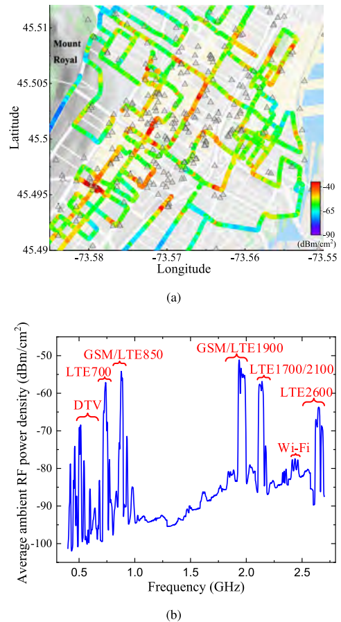
FIGURE 4. (a) Ambient RF power density of GSM/LTE 1900 band in downtown Montreal [41]. The triangle symbol marks the cellular base station and (b) average ambient RF power density in downtown Montreal across a frequency band from 400 MHz to 2.7 GHz [41].
