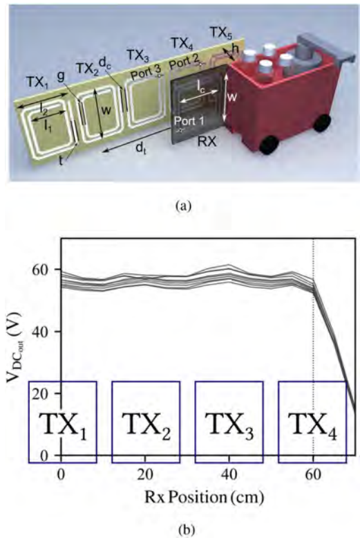
FIGURE 24. (a) Pictorial representation of the link setup and (b) measured dc-output voltage with respect to different positions of the receiving coil, as presented in [154] © IEEE 2017.
